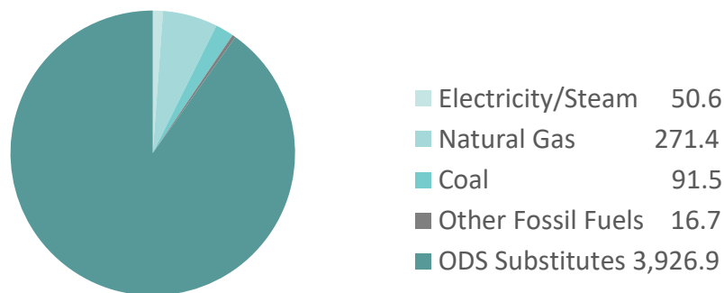
FIGURE 8: INDUSTRIAL EMISSIONS BY SOURCE (MTCO 2 e)
