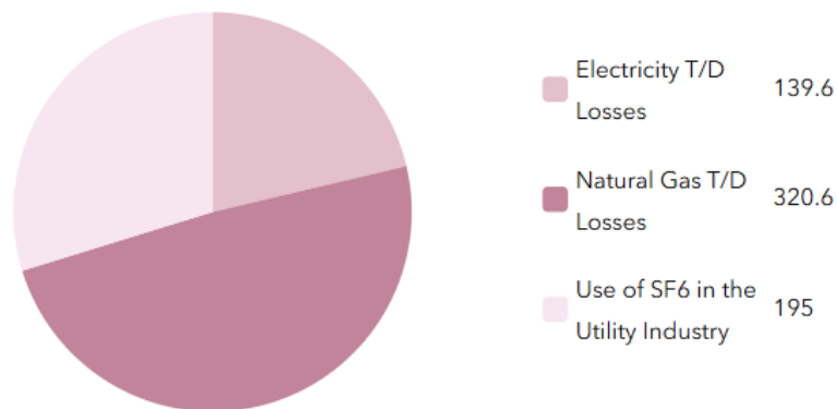
FIGURE 10: ENERGY DISTRIBUTION EMISSIONS BY SOURCE (MTCO 2 e)
