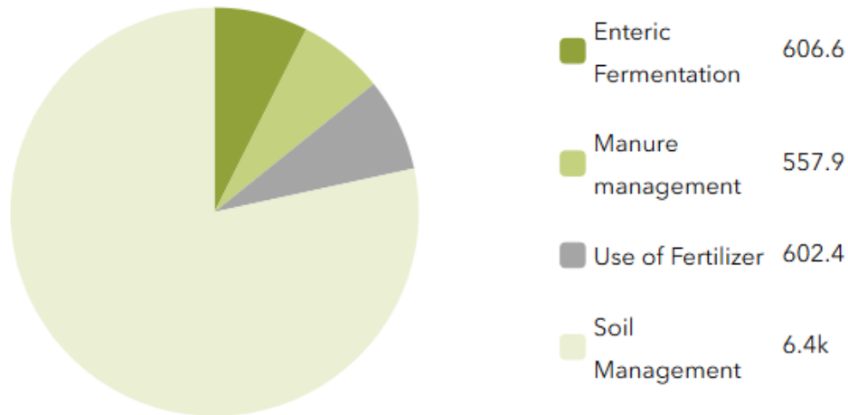
FIGURE 11: AGRICULTURAL EMISSIONS BY SOURCE (MTCO 2 e)
