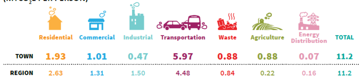
FIGURE 3. NEWFANE’S PER CAPITA ENERGY CONSUMPTION
