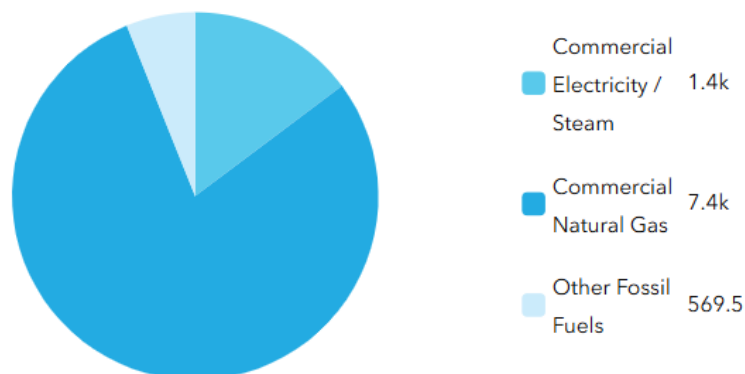
FIGURE 7: COMMERCIAL EMISSIONS BY SOURCE (MTCO 2 e)
