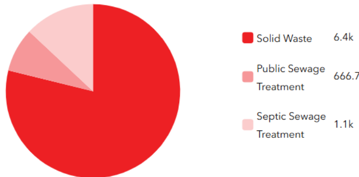
FIGURE 9: WASTE MANAGMENT EMISSIONS BY SOURCE (MTCO 2 e)
