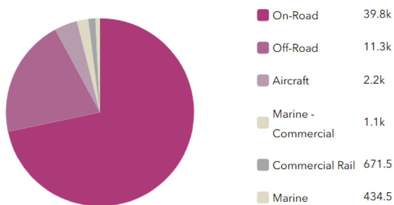
FIGURE 4: TRANSPORTATION EMISSIONS BY SOURCE (MTCO2e)
