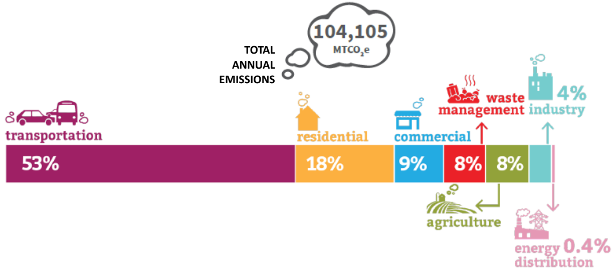
FIGURE 2: NEWFANE’S PER CAPITA EMISSIONS
