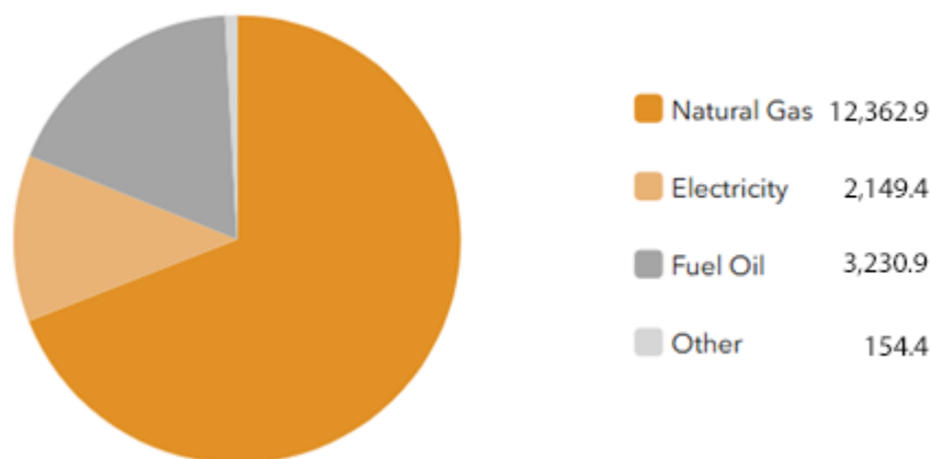
FIGURE 5: RESIDENTIAL EMISSIONS BY SOURCE (MTCO 2 e)
